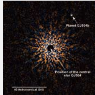
The 4 Jupiter mass planet GJ504b taken with Subaru telescope
