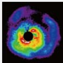
Infrared Picture of the planet forming region (Protoplanetary Disk) taken by Subaru Telescope. In such a disk the life in the universe may be born.
