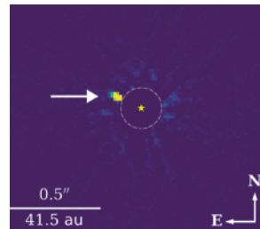
Discovered giant gas planet HIP 54515 b (white arrow)
