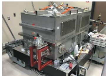
Instrument for habitable exoplanet search, Infrared Doppler spectrometer IRD.
